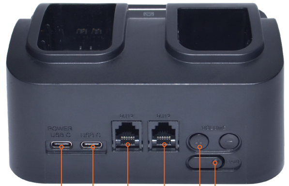
USB-C port for power USB-C port for data-in RJ12 port RJ12 port Pairing switch Volume up/down
